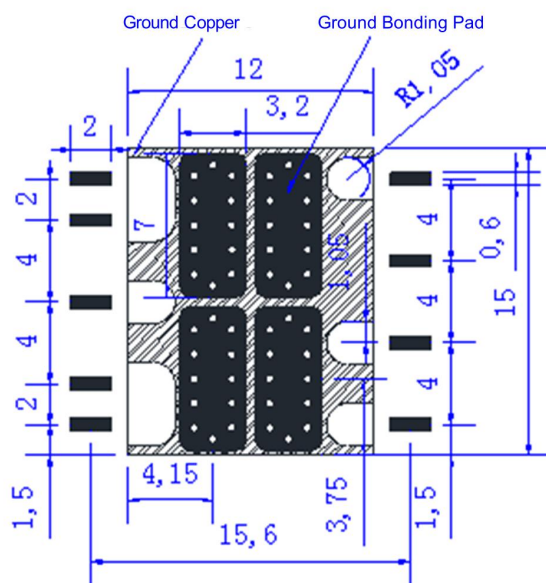
Dimension(unit: mm)
