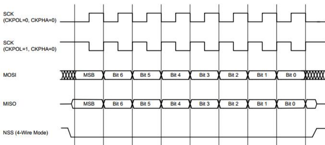
Figure 17.6. Slave Mode Data/Clock Timing (CKPHA = 0)
